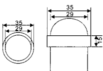
DS-20 Door stopper Material: Stainless steel Finishes: SSS, PSS
