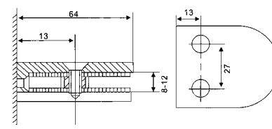
GC-23 Material: Stainless steel Finishes: SSS, PSS
