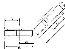
GC-22 Material: Stainless steel Finishes: SSS, PSS
