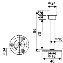
DS-01 Door stopper Material: Stainless steel Finishes: SSS, PSS
