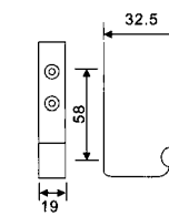
DS-40 Door stopper with hook Material: Stainless steel Finishes: SSS, PSS
