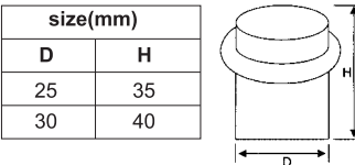
DS-06 Door stopper Material: Stainless steel Finishes: SSS, PSS
