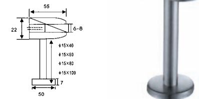
GC-30 Material: Stainless steel Finishes: SSS, PSS Size: 33x55mm, 43x65mm 55x73mm Suited Thickness: 6-8mm 10-12mm 12-15mm
