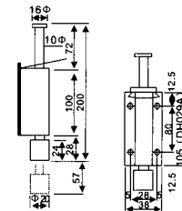
DS-40 Door stopper with hook Material: Stainless steel Finishes: SSS, PSS
