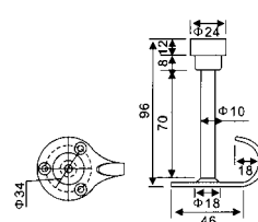
DS-02 Door stopper with hook Material: Stainless steel Finishes: SSS, PSS
