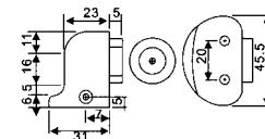
DS-24 Magnetic door holder Material: Stainless steel, Zinc alloy Finishes: SSS, PSS, AB, AC, SN, SCP, CP
