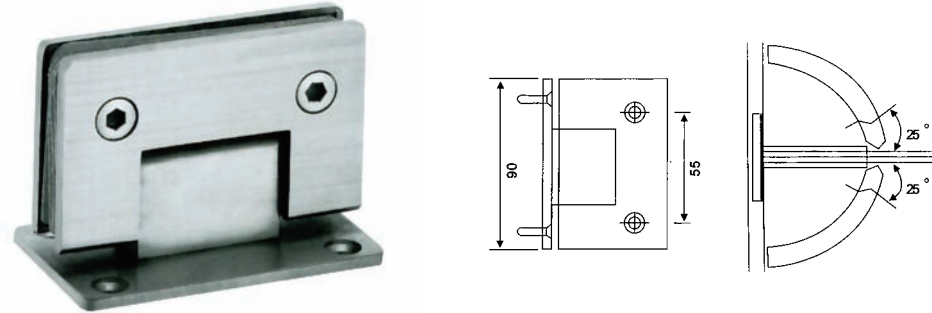
GC-16 Shower door hinge Material: Stainless steel Finishes: SSS, PSS
