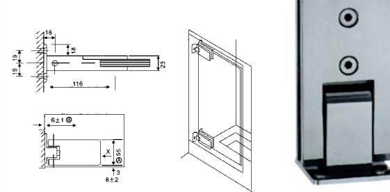
GC-19 Shower door hinge Material: Stainless steel Finishes: SSS, PSS
