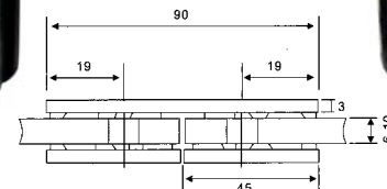
GC-23 Material: Stainless steel Finishes: SSS, PSS
