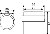
DS-19 Door stopper Material: Stainless steel, Zinc alloy Finishes: SSS, PSS, SN, SCP, PB, AB, AC, BN
