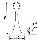
DS-25 Magnetic door holder Material: Stainless steel, Zinc alloy Finishes: SSS, PSS, AB, AC, SN, SCP, CP
