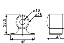
DS-23 Magnetic door holder Material: Zinc alloy Finishes: SCP, CP, AB, AC, SN
