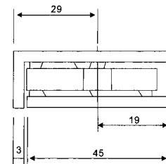
GC-08 Glass clip(Glass to glass) Material: Stainless steel Finishes: SSS, PSS Thickness: 2.5mm, 3mm, 3.5mm
