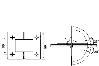
GC-18 Shower door hinge Material: Stainless steel Finishes: SSS, PSS
