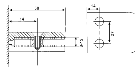
GC-26 Material: Zinc alloy Finishes: CP, BN
