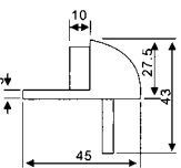
DS-16 Door stopper Material: Zinc alloy, Stainless steel Finishes: SCP, CP, SN, AB, AC, SSS, PSS
