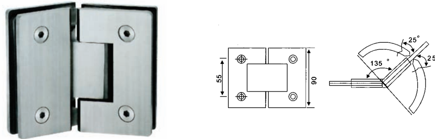
GC-19 Shower door hinge Material: Stainless steel Finishes: SSS, PSS
