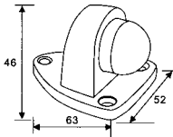
DS-41 Door stopper Material: Zinc alloy Finishes: SCP, CP, AB, AC, SN
