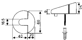
DS-17 Door stopper Material: Zinc alloy, Stainless steel Finishes: SSS, PSS, AB, AC, SN, SCP, CP
