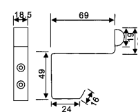
DS-22 Door stopper with hook Material: Stainless steel Finishes: SSS, PSS
