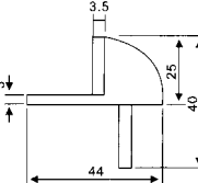
DS-13 Door stopper Material: Stainless steel Finishes: SSS, PSS
