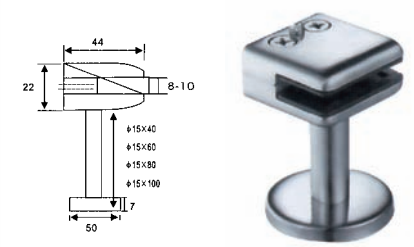
GC-29 Material: Stainless steel Finishes: SSS, PSS
