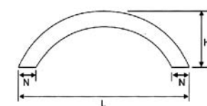
FH016 Hollow stainless steel furniture handle
