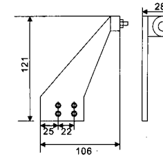
DS-39 Door stopper Material: Stainless steel Finishes: SSS, PSS
