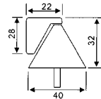
DS-07 Door stopper Material: Zinc alloy Finishes: SCP, CP, SN, PB, AB, AC
