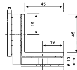
GC-09 Glass clip(Glass to glass) Material: Stainless steel Finishes: SSS, PSS Thickness: 2.5mm, 3mm, 3.5mm
