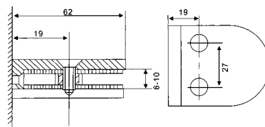
GC-24 Material: Stainless steel Finishes: SSS, PSS
