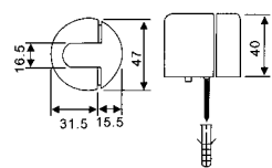
DS-18 Door stopper Material: Zinc alloy, Stainless steel Finishes: SCP, CP, AB, AC, SN, SSS, PSS
