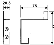
DS-29 Door stopper with hook Material: Stainless steel Finishes: SSS, PSS
