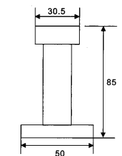
DS-31 Door stopper Material: Stainless steel Finishes: SSS, PSS
