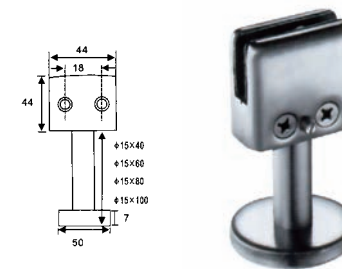
GC-27 Material: Stainless steel Finishes: SSS, PSS
